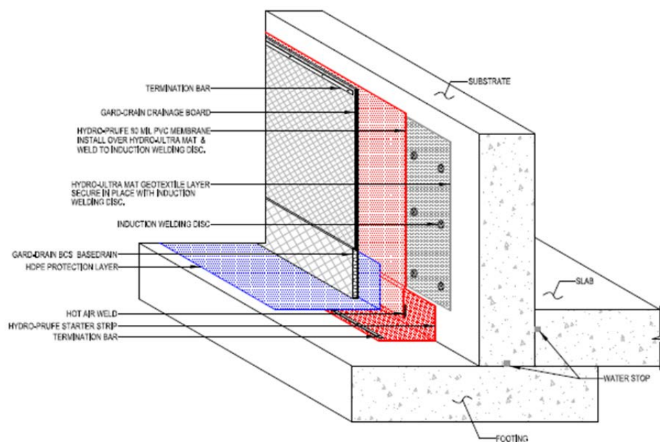
FIGURE 1—TYPICAL MEMBRANE INSTALLATION DETAIL
