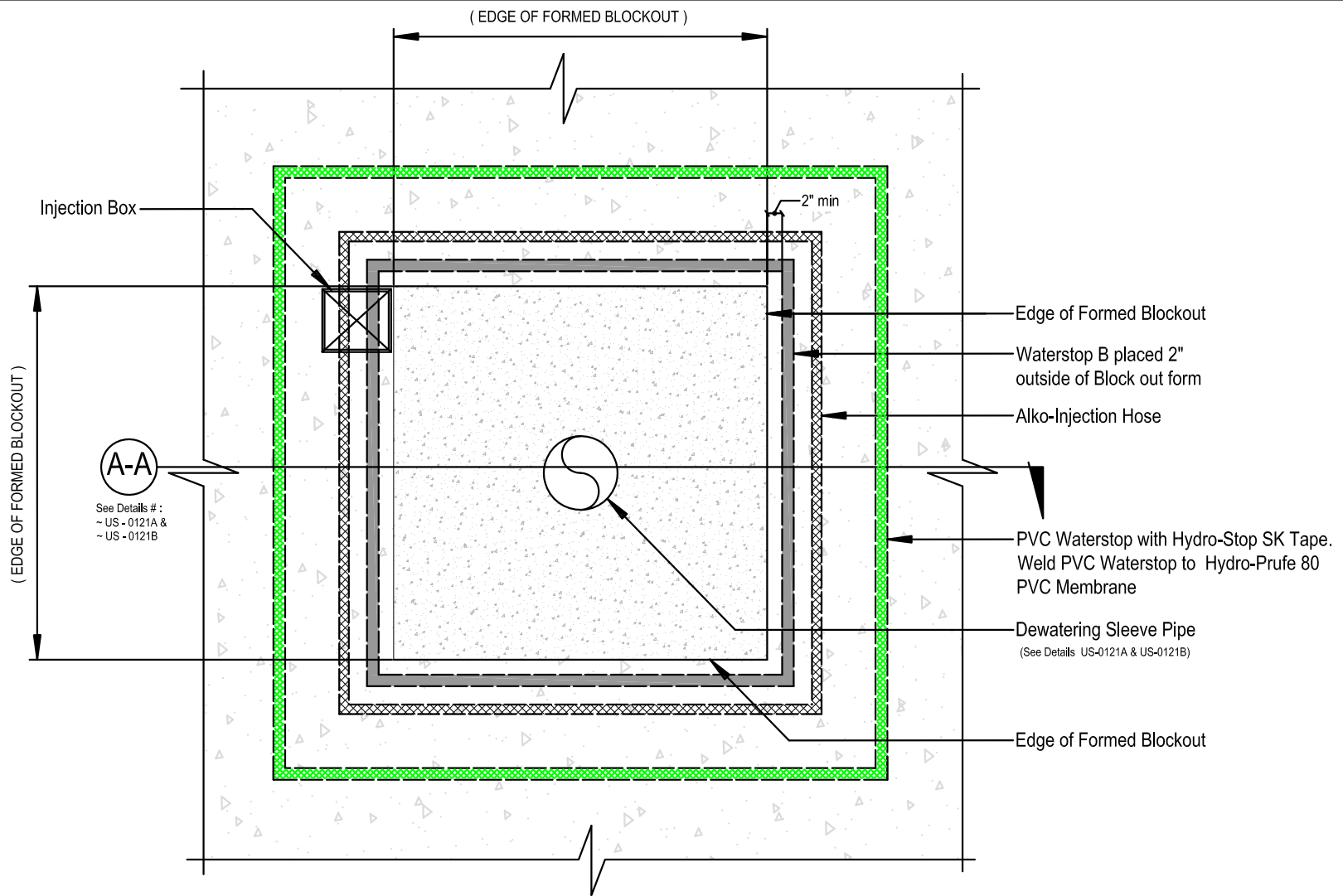
PLAN VIEW ( EDGE OF FORMED BLOCKOUT )
